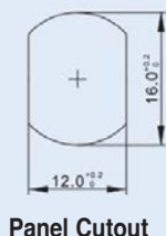
Panel Cutout
